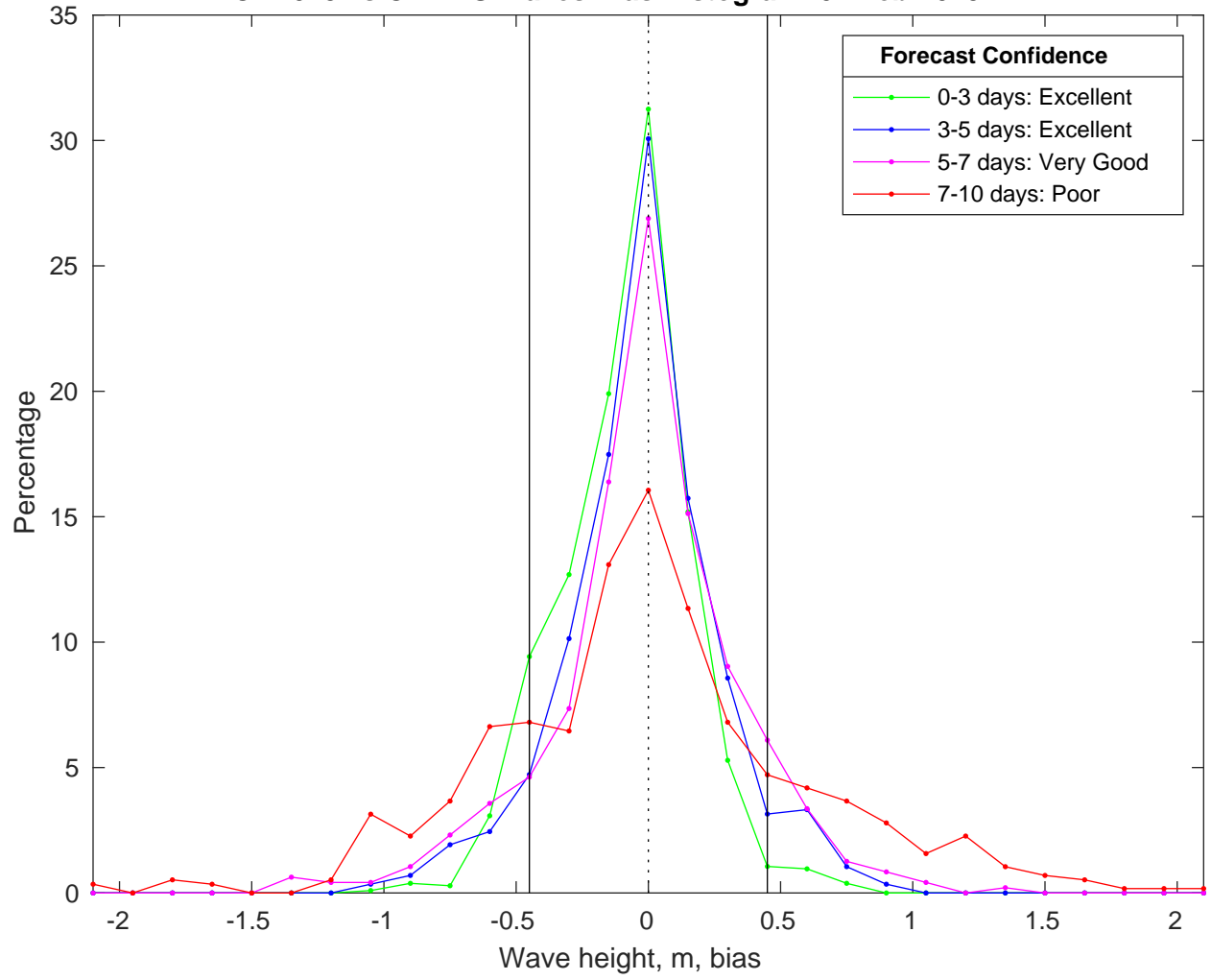
NDBC 41013 vs CMEMS Waves Bias Histogram: 07-Feb-2025
