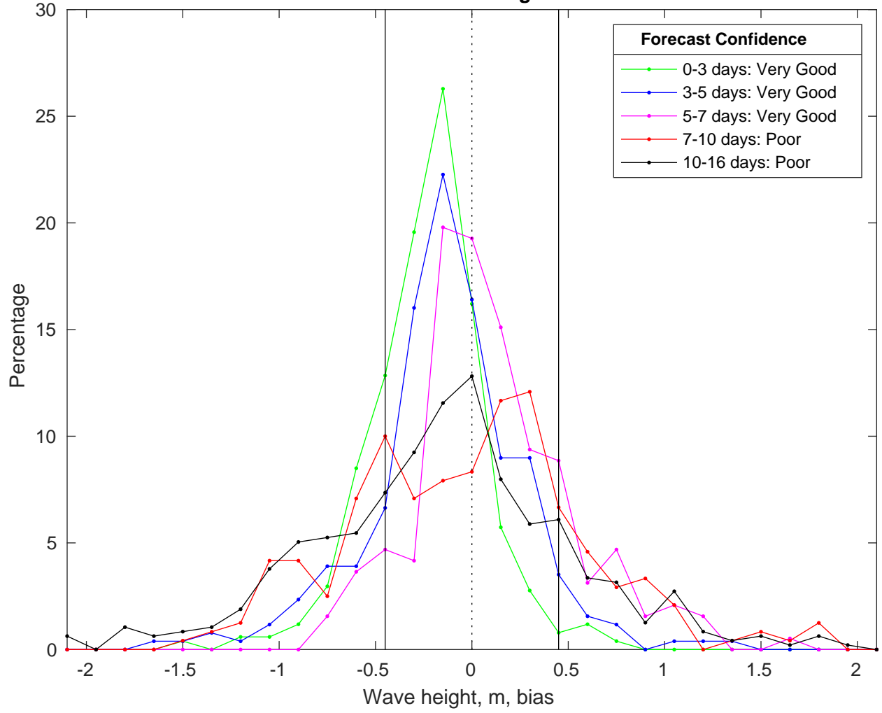
NDBC 41013 vs GFS Waves Bias Histogram: 07-Feb-2025
