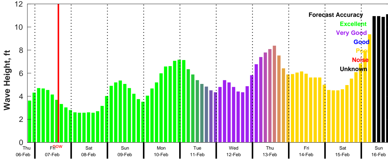
CMEMS Wave Forecast for NDBC 41013 from 06-Feb-2025 19:00:00 to 16-Feb-2025 19:00:00
