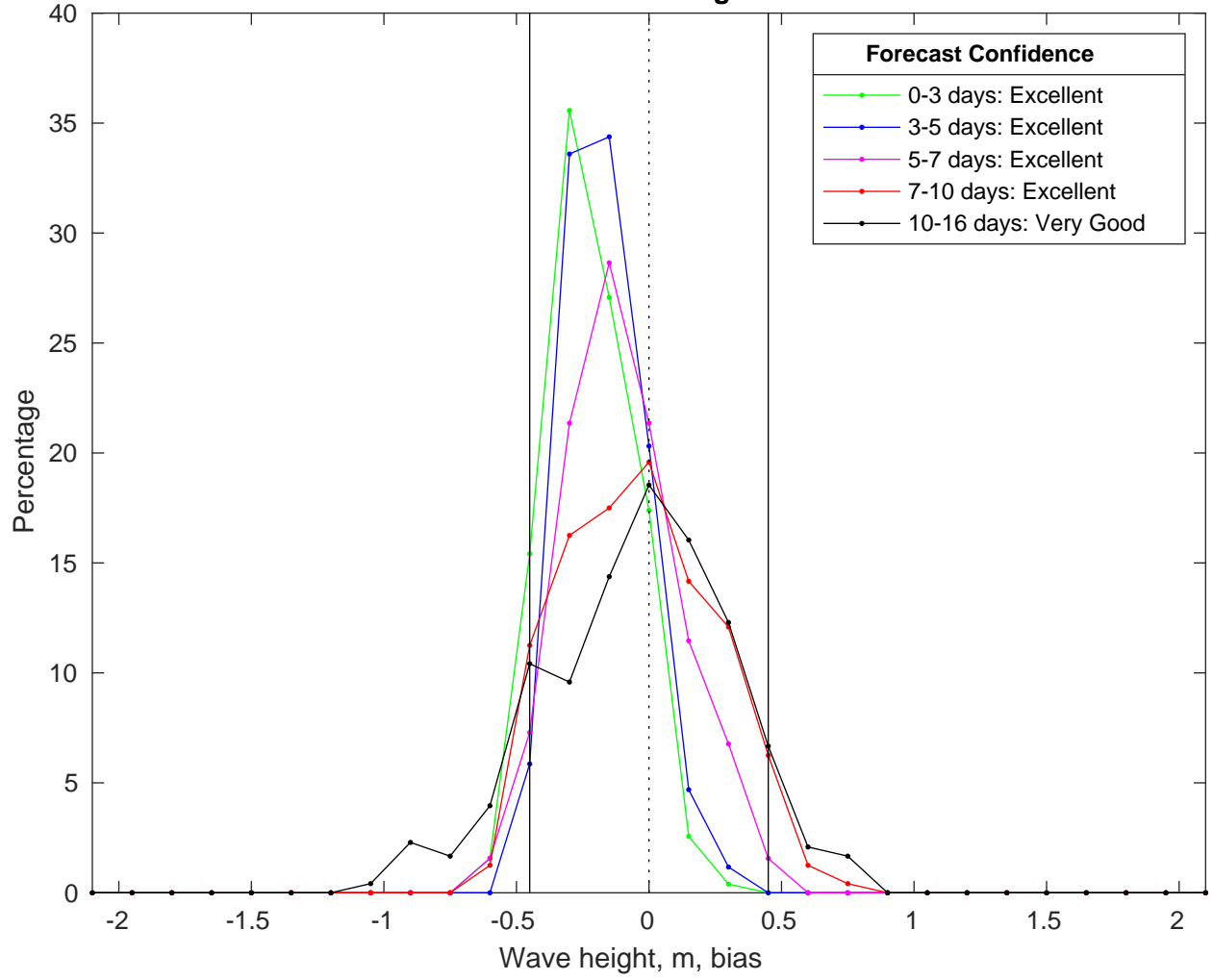
NDBC 41040 vs GFS Waves Bias Histogram: 07-Feb-2025
