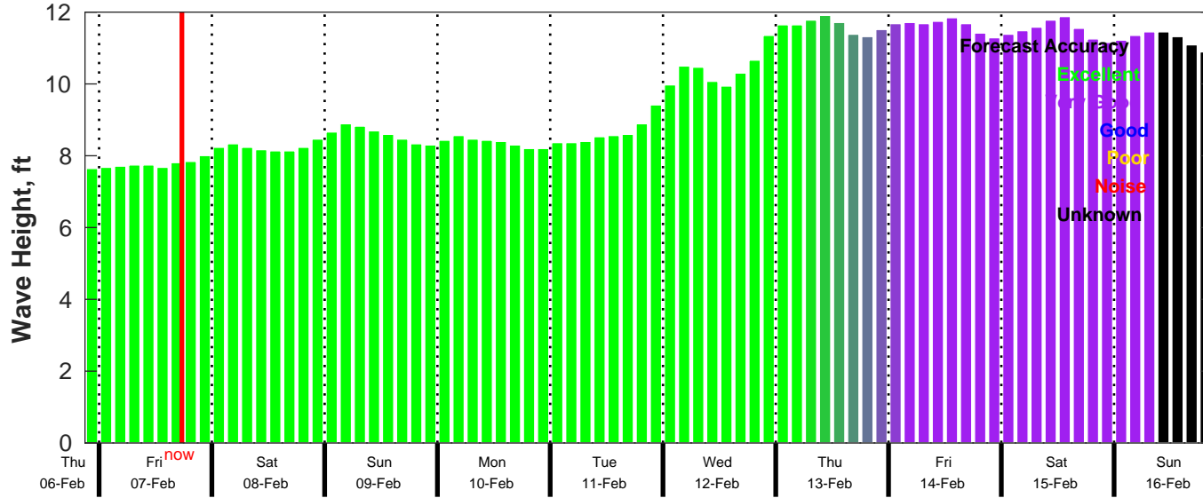
CMEMS Wave Forecast for NDBC 41040 from 06-Feb-2025 21:00:00 to 16-Feb-2025 21:00:00
