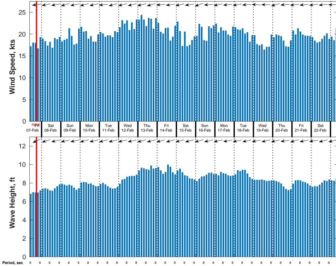
Wind & Wave Forecast for NDBC 41040 from 07-Feb-2025 09:00:00 to 23-Feb-2025 09:00:00
