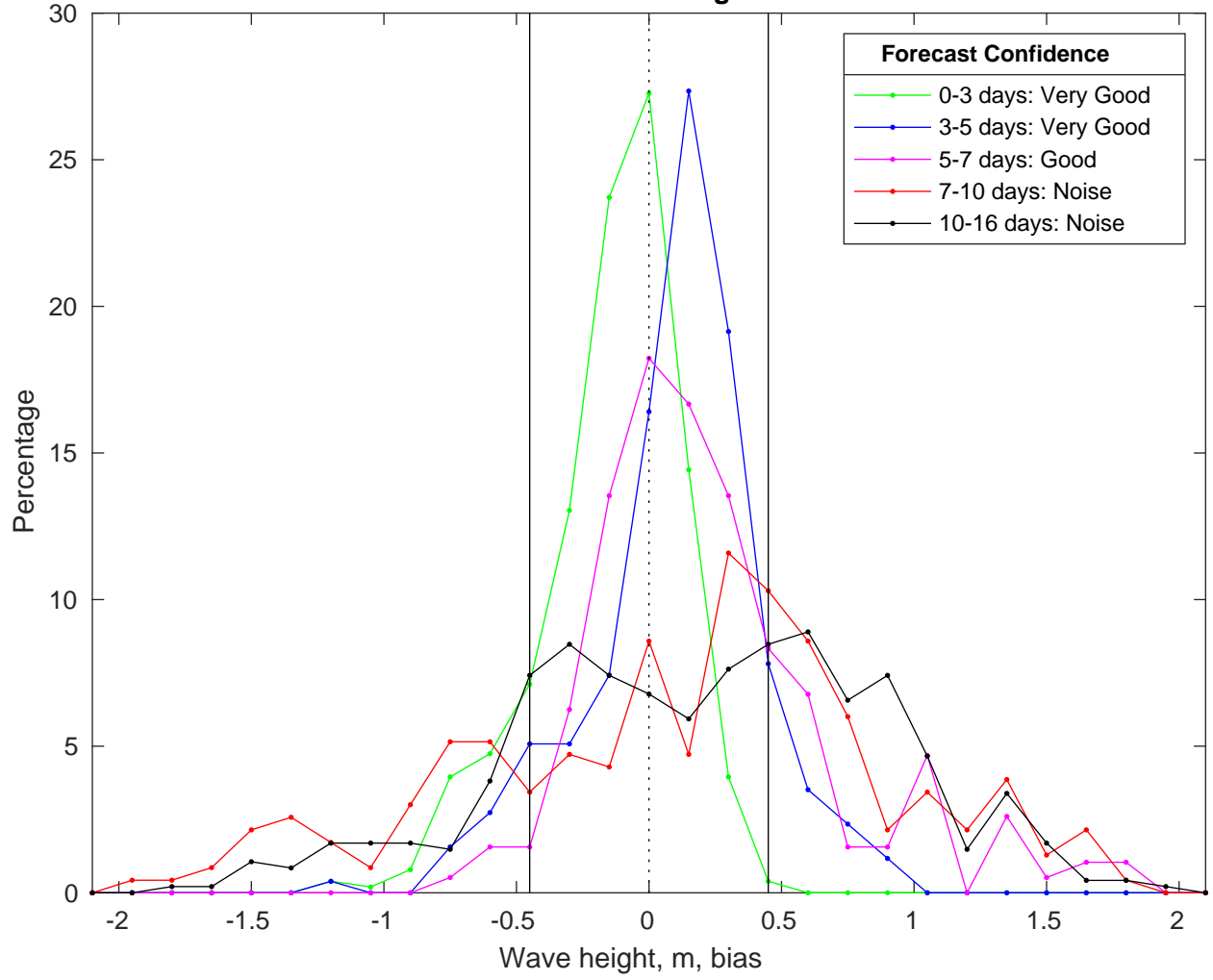
NDBC 42019 vs GFS Waves Bias Histogram: 07-Feb-2025
