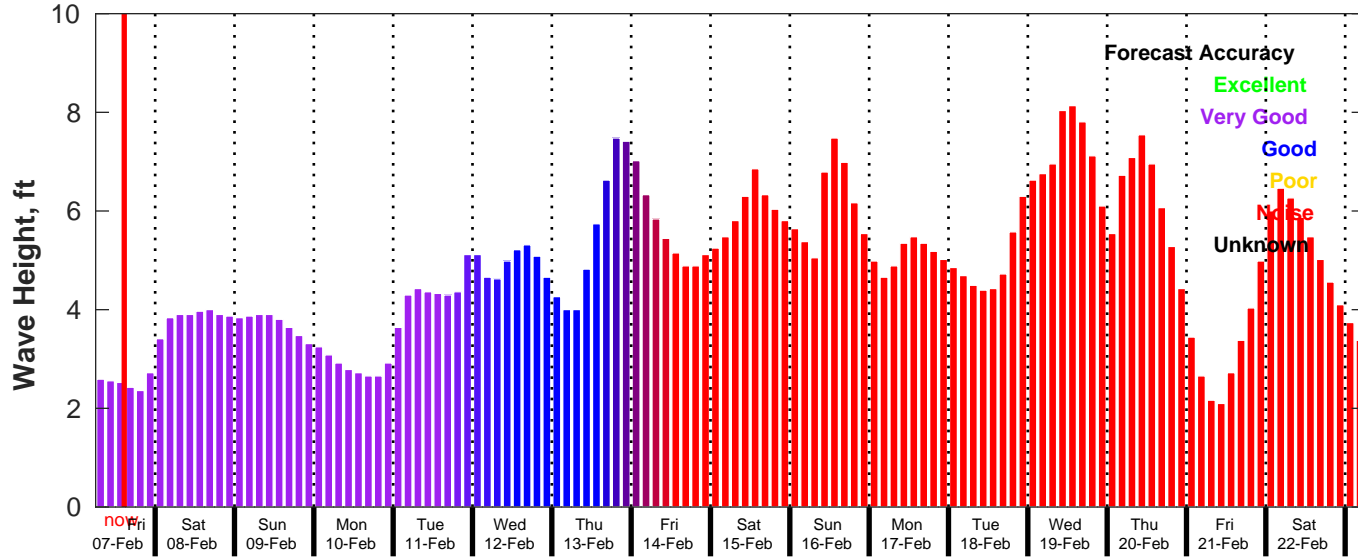
GFS Wave Forecast for NDBC 42019 from 07-Feb-2025 06:00:00 to 23-Feb-2025 06:00:00
