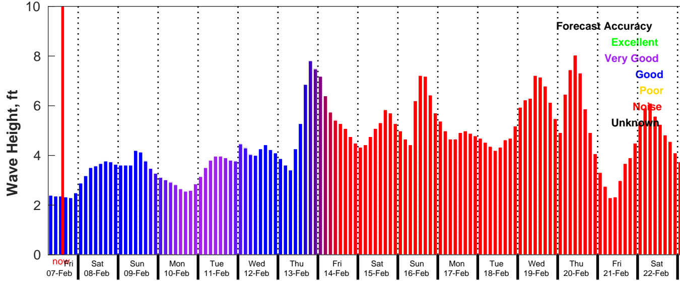
GFS Wave Forecast for NDBC 42020 from 07-Feb-2025 06:00:00 to 23-Feb-2025 06:00:00
