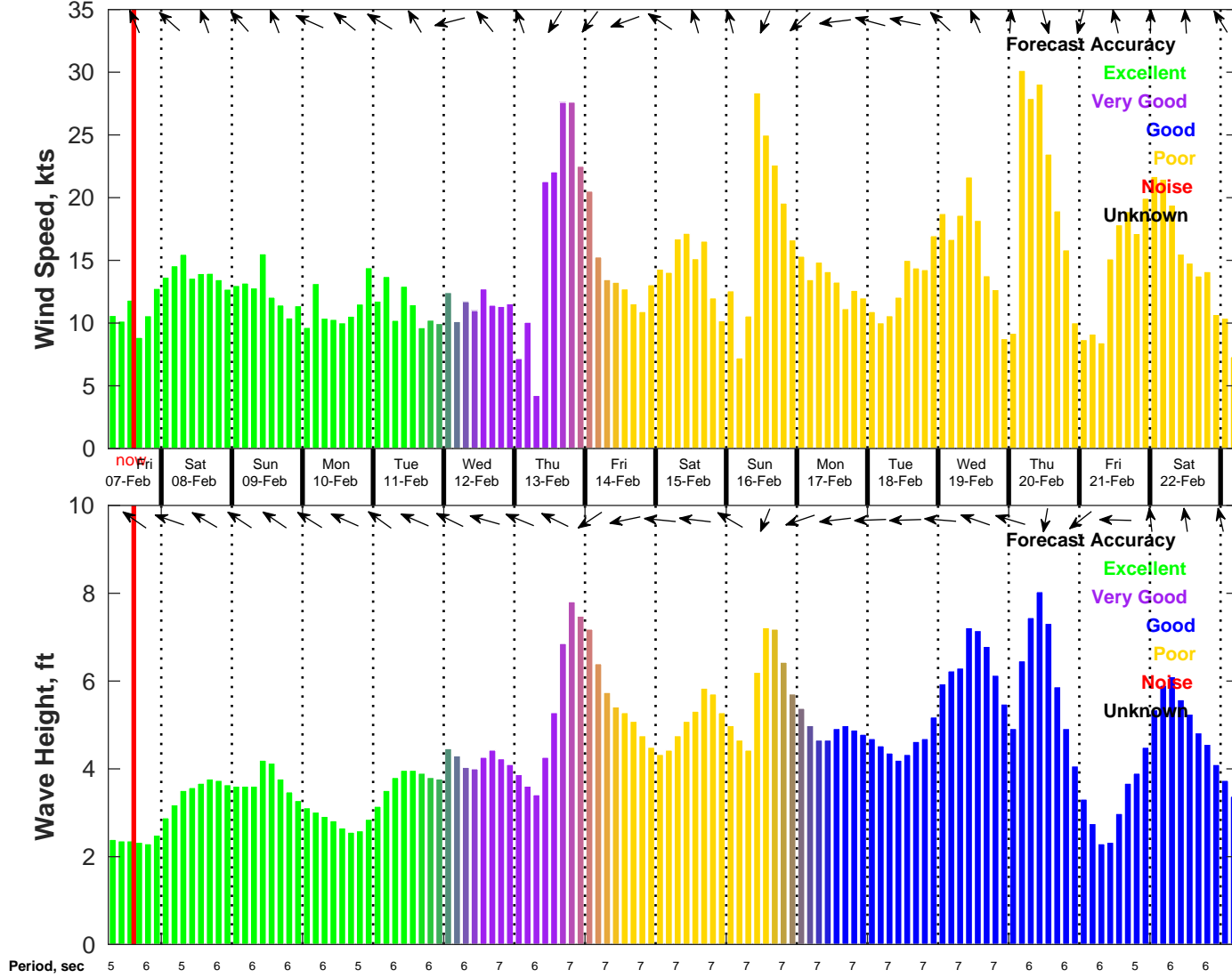
Wind & Wave Forecast for NDBC 42020 from 07-Feb-2025 06:00:00 to 23-Feb-2025 06:00:00
