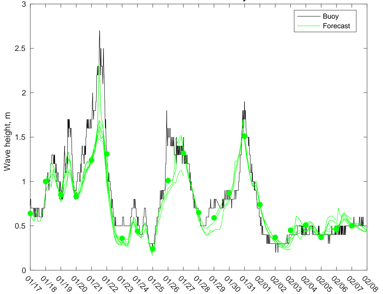
NDBC 42035 vs CMEMS Waves: 0 to 3 day forecast
