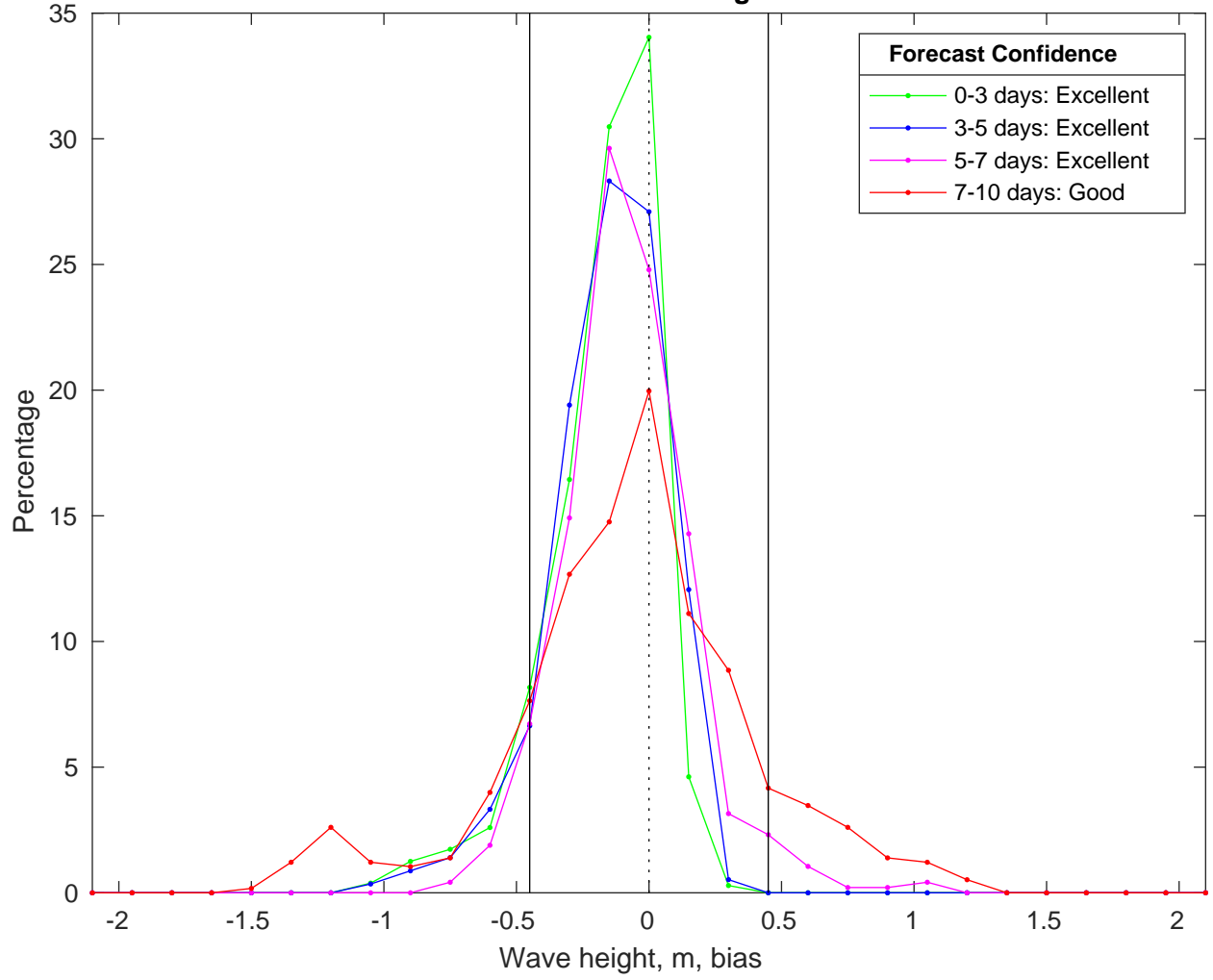
NDBC 42035 vs CMEMS Waves Bias Histogram: 07-Feb-2025
