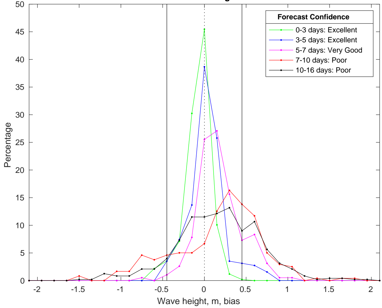
NDBC 42035 vs GFS Waves Bias Histogram: 07-Feb-2025
