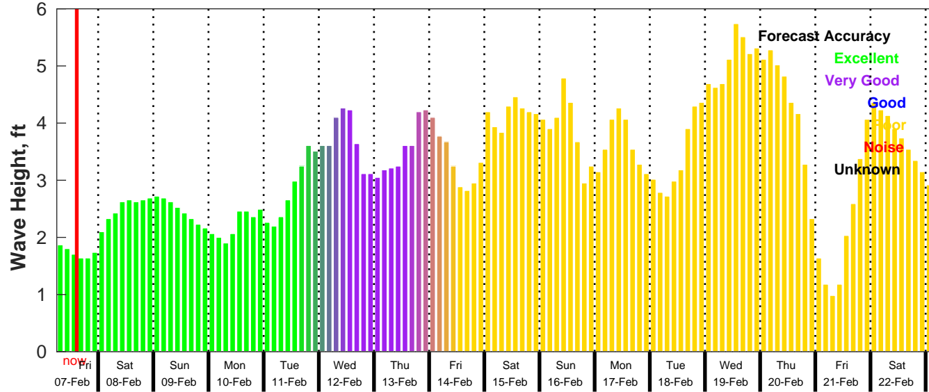
GFS Wave Forecast for NDBC 42035 from 07-Feb-2025 06:00:00 to 23-Feb-2025 06:00:00
