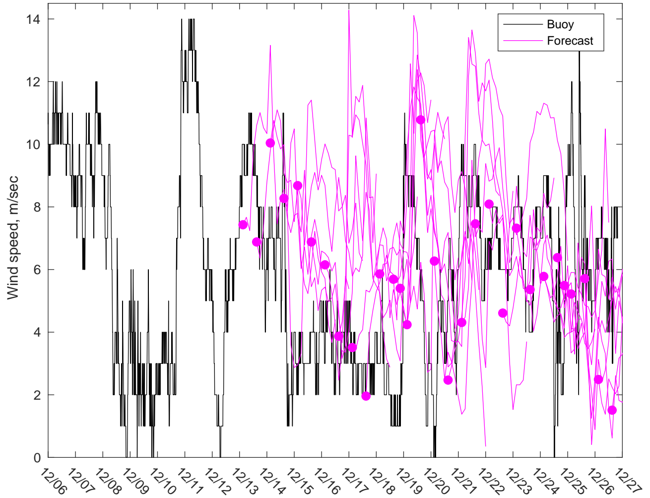
NDBC 42035 vs GFSWinds: 7 to 10 day forecast
