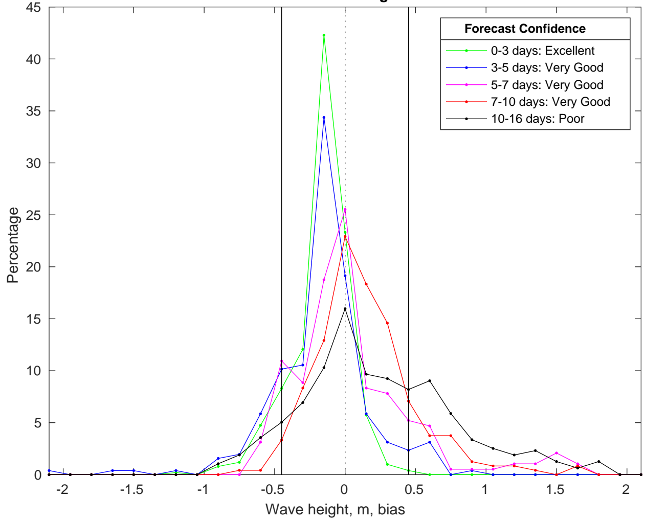
NDBC 42036 vs GFS Waves Bias Histogram: 07-Feb-2025
