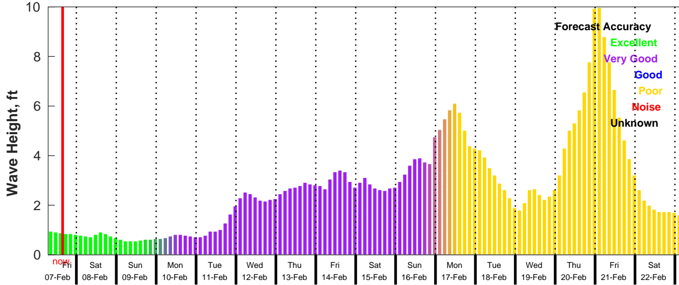
GFS Wave Forecast for NDBC 42036 from 07-Feb-2025 07:00:00 to 23-Feb-2025 07:00:00
