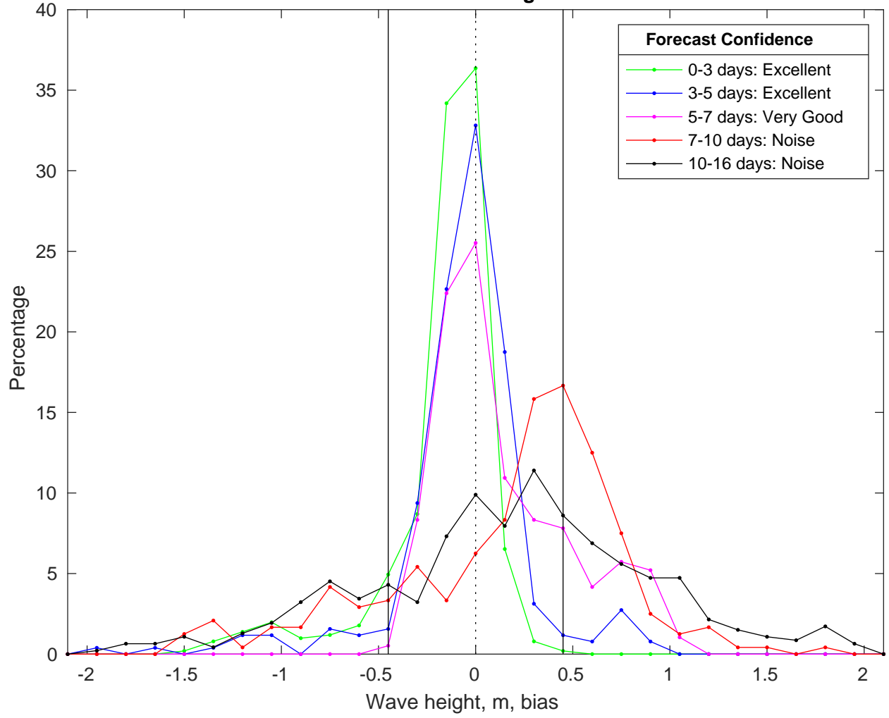
NDBC 42040 vs GFS Waves Bias Histogram: 07-Feb-2025
