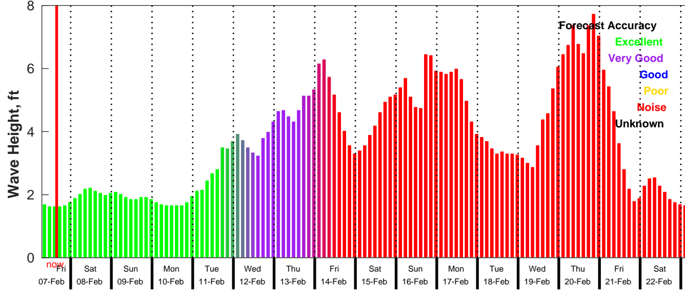
GFS Wave Forecast for NDBC 42040 from 07-Feb-2025 07:00:00 to 23-Feb-2025 07:00:00
