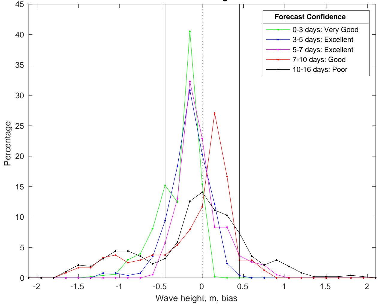
NDBC 42084 vs GFS Waves Bias Histogram: 07-Feb-2025
