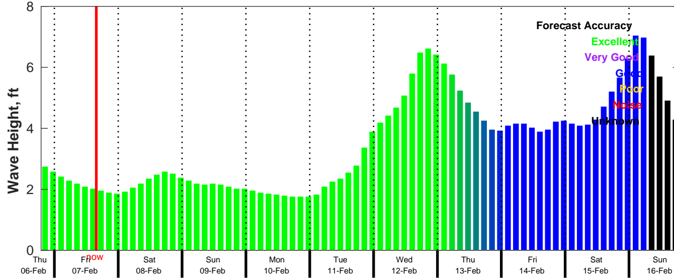
CMEMS Wave Forecast for NDBC 42084 from 06-Feb-2025 19:00:00 to 16-Feb-2025 19:00:00
