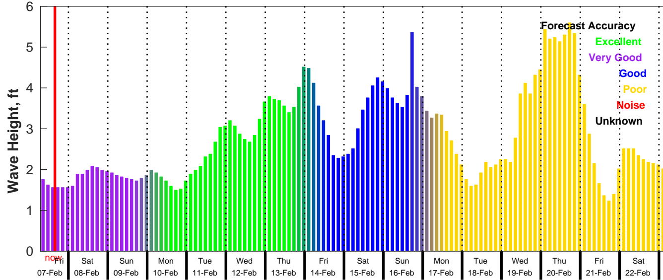
GFS Wave Forecast for NDBC 42084 from 07-Feb-2025 07:00:00 to 23-Feb-2025 07:00:00
