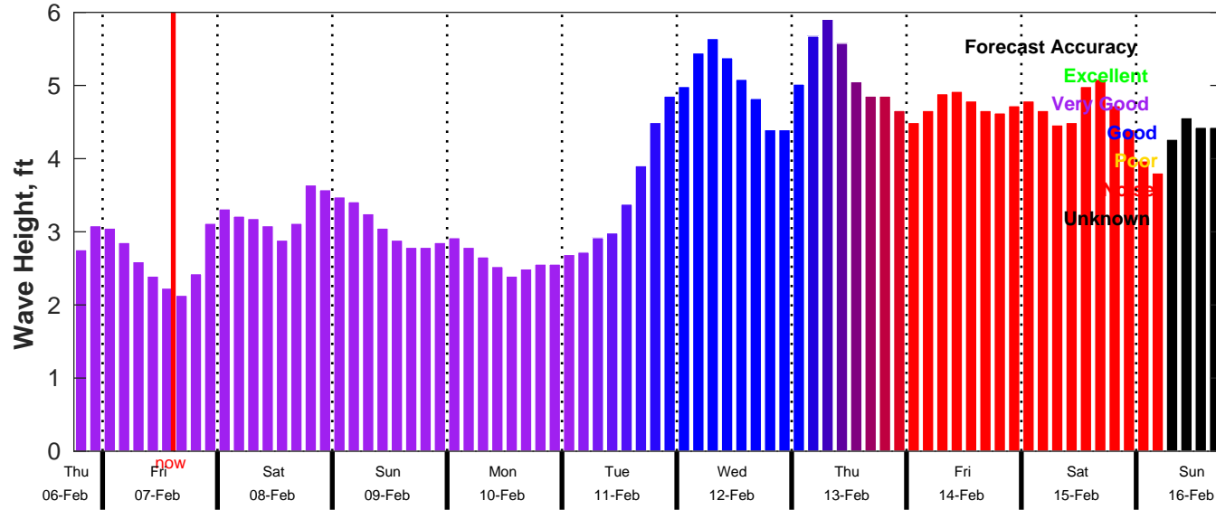
CMEMS Wave Forecast for NDBC 42092 from 06-Feb-2025 18:00:00 to 16-Feb-2025 18:00:00
