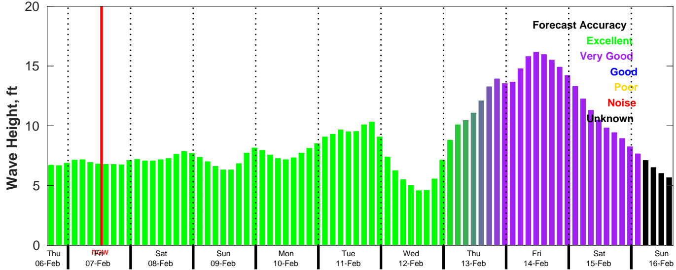
CMEMS Wave Forecast for NDBC 46011 from 06-Feb-2025 16:00:00 to 16-Feb-2025 16:00:00
