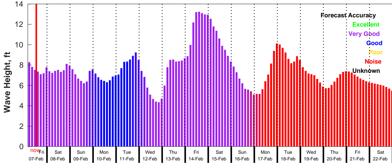
GFS Wave Forecast for NDBC 46011 from 07-Feb-2025 04:00:00 to 23-Feb-2025 04:00:00
