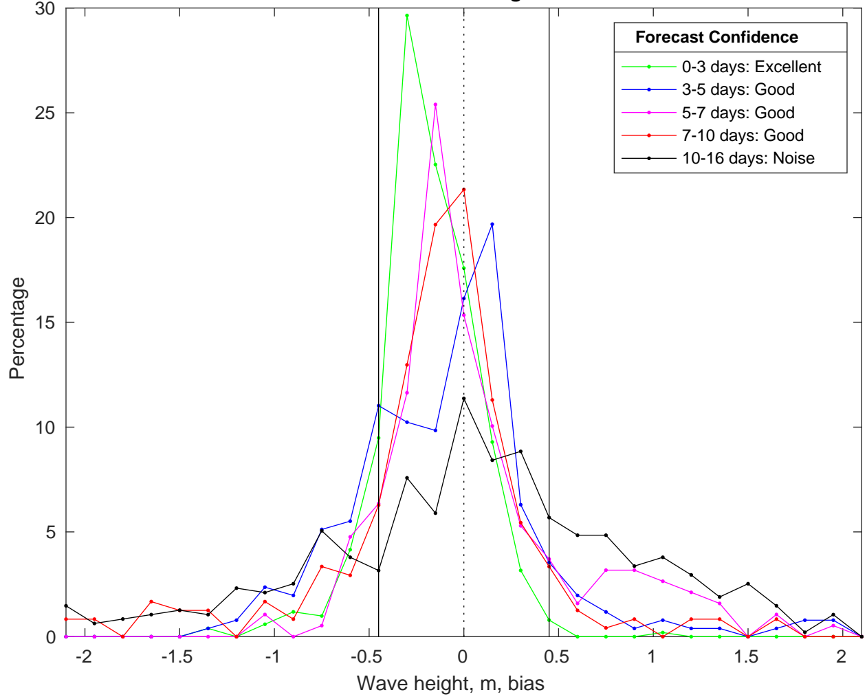
NDBC 46028 vs GFS Waves Bias Histogram: 07-Feb-2025
