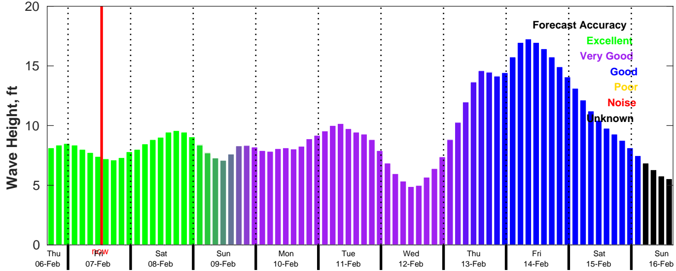
CMEMS Wave Forecast for NDBC 46028 from 06-Feb-2025 16:00:00 to 16-Feb-2025 16:00:00
