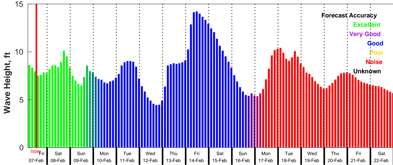
GFS Wave Forecast for NDBC 46028 from 07-Feb-2025 04:00:00 to 23-Feb-2025 04:00:00
