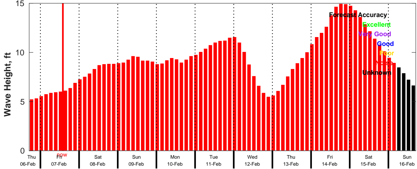
CMEMS Wave Forecast for NDBC 46053 from 06-Feb-2025 17:00:00 to 16-Feb-2025 17:00:00
