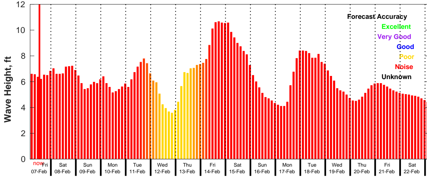
GFS Wave Forecast for NDBC 46054 from 07-Feb-2025 04:00:00 to 23-Feb-2025 04:00:00
