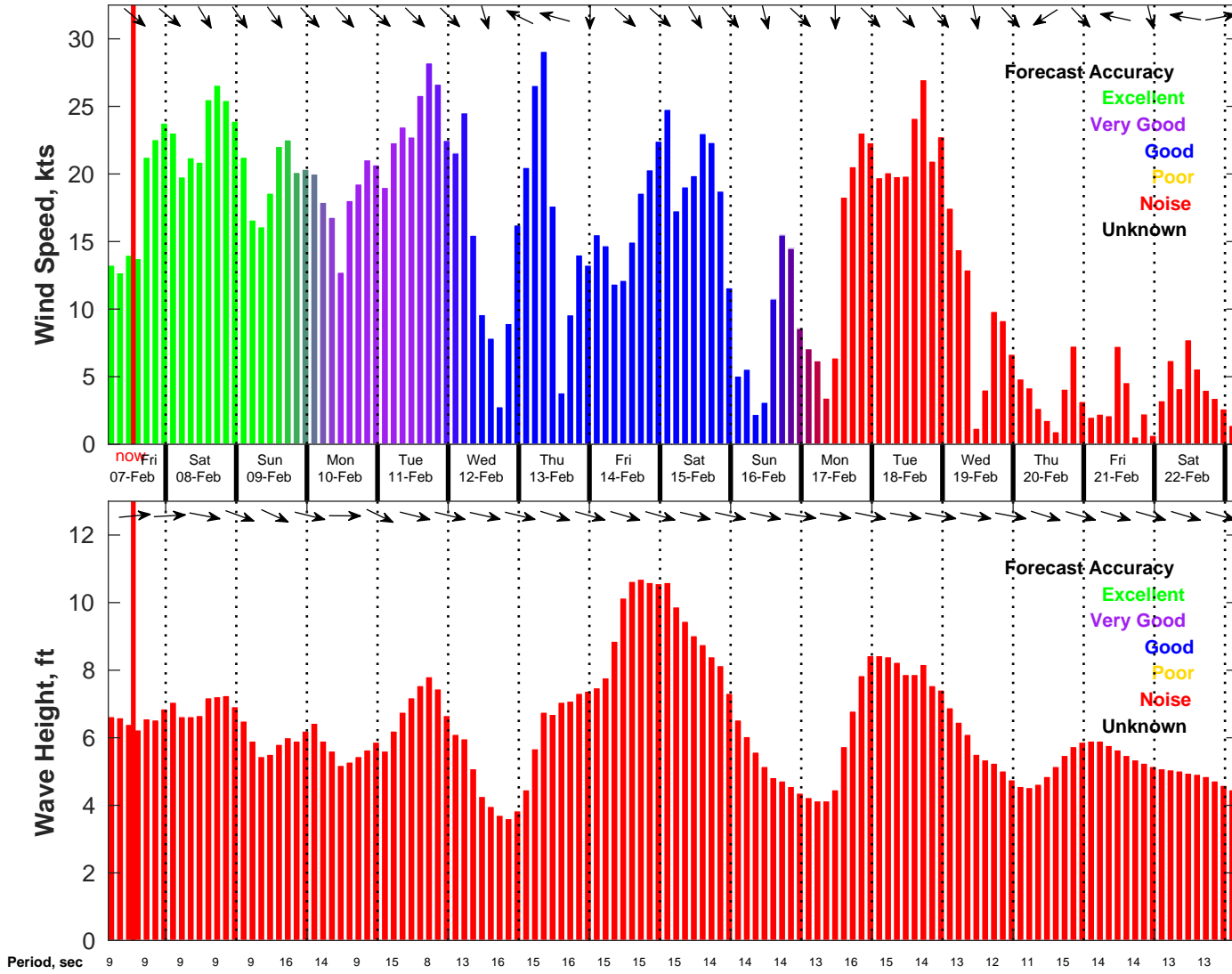
Wind & Wave Forecast for NDBC 46054 from 07-Feb-2025 04:00:00 to 23-Feb-2025 04:00:00
