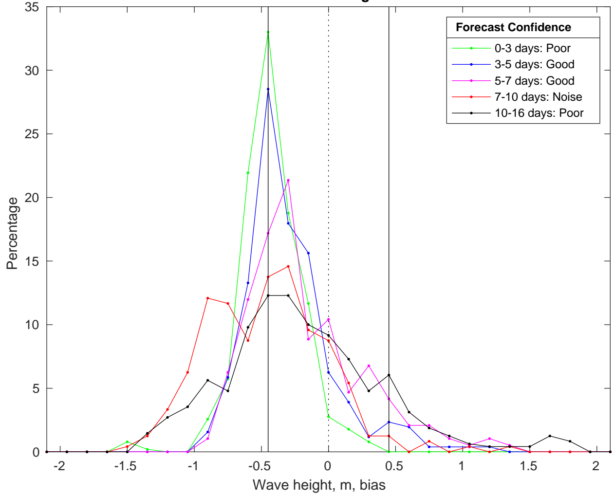
NDBC 46069 vs GFS Waves Bias Histogram: 07-Feb-2025
