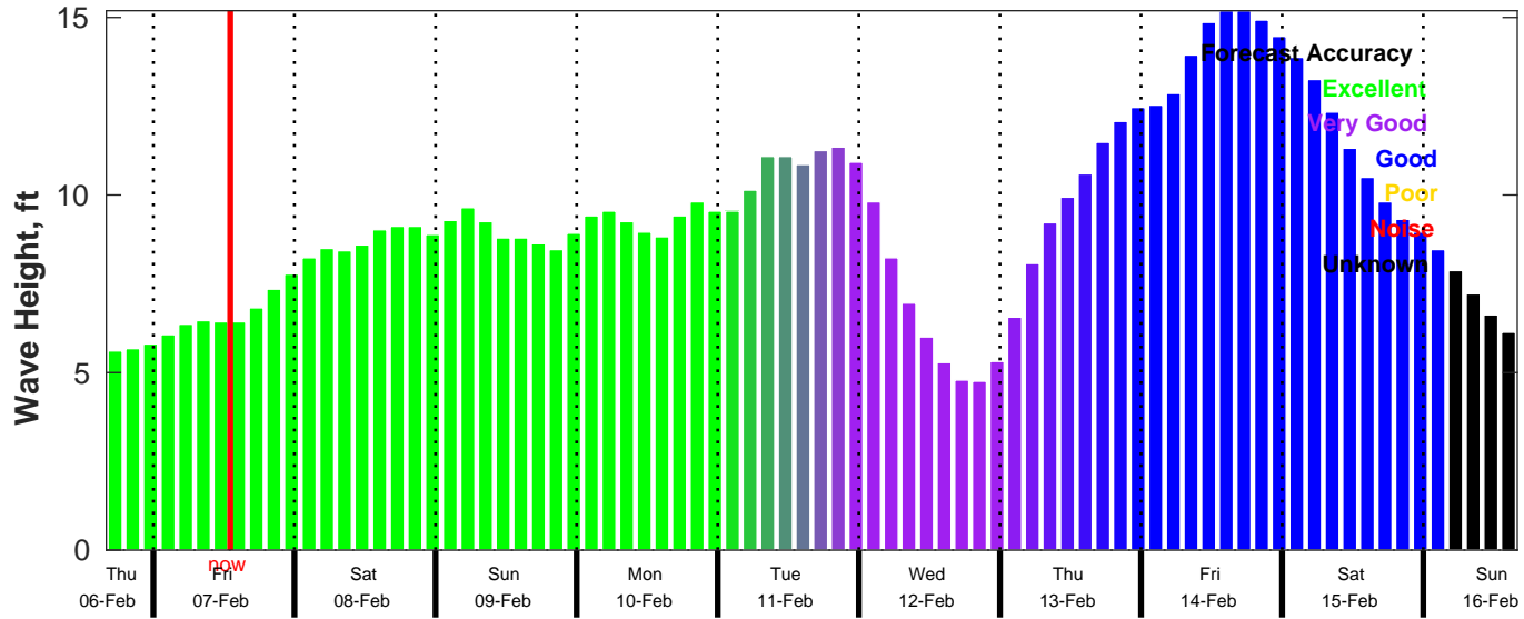
CMEMS Wave Forecast for NDBC 46069 from 06-Feb-2025 16:00:00 to 16-Feb-2025 16:00:00
