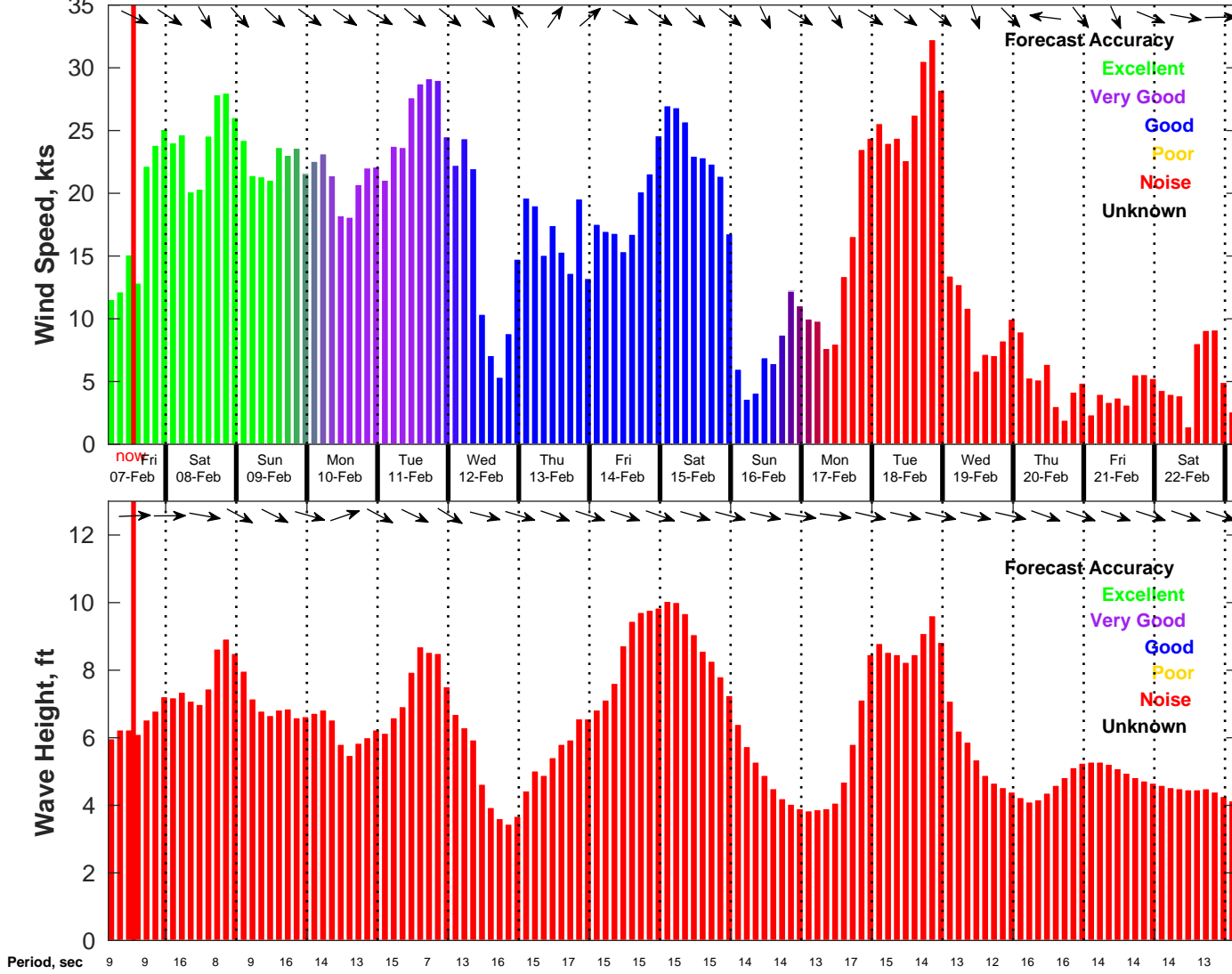
Wind & Wave Forecast for NDBC 46069 from 07-Feb-2025 04:00:00 to 23-Feb-2025 04:00:00
