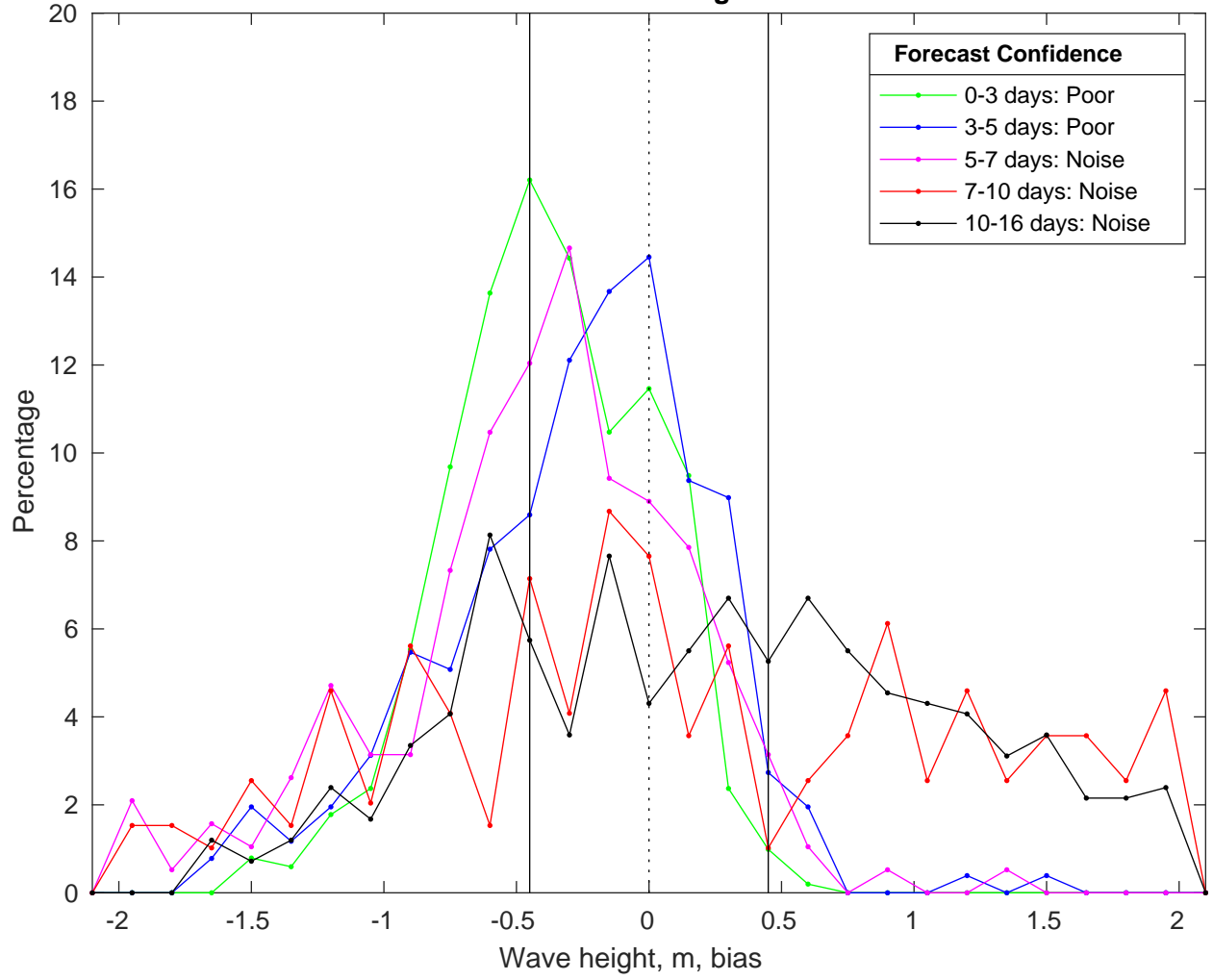
NDBC 46246 vs GFS Waves Bias Histogram: 07-Feb-2025
