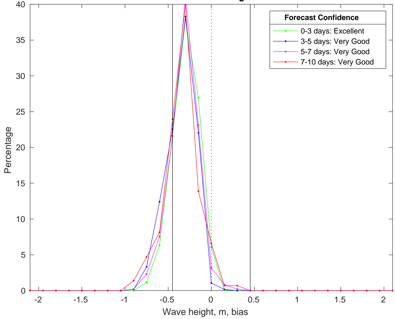
NDBC 51209 vs CMEMS Waves Bias Histogram: 07-Feb-2025
