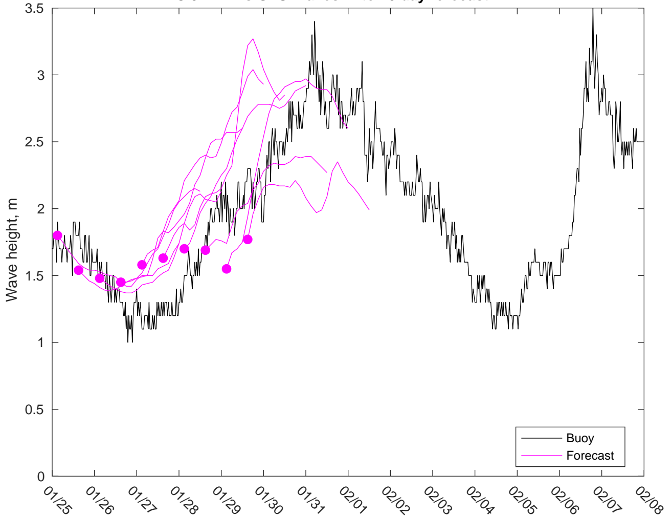
NDBC 52211 vs GFS Waves: 7 to 10 day forecast
