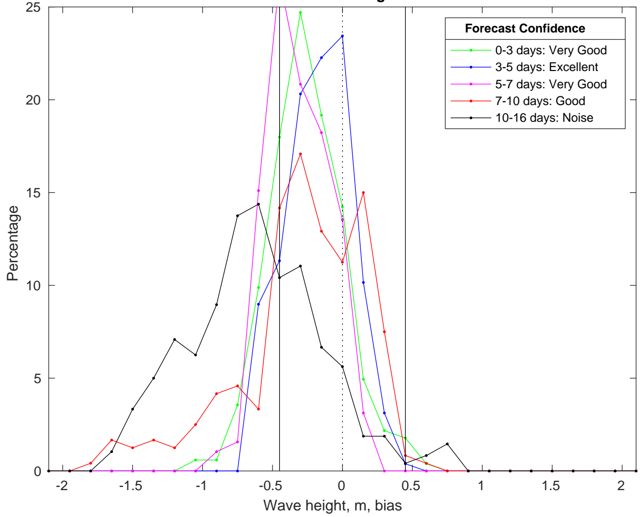
NDBC 52212 vs GFS Waves Bias Histogram: 07-Feb-2025
