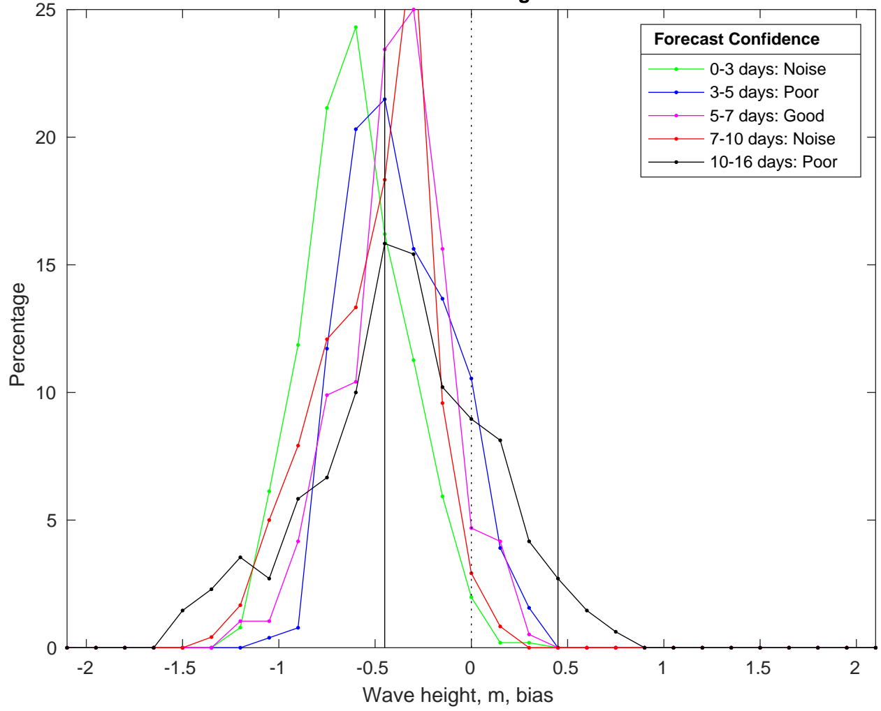
NDBC 52213 vs GFS Waves Bias Histogram: 07-Feb-2025
