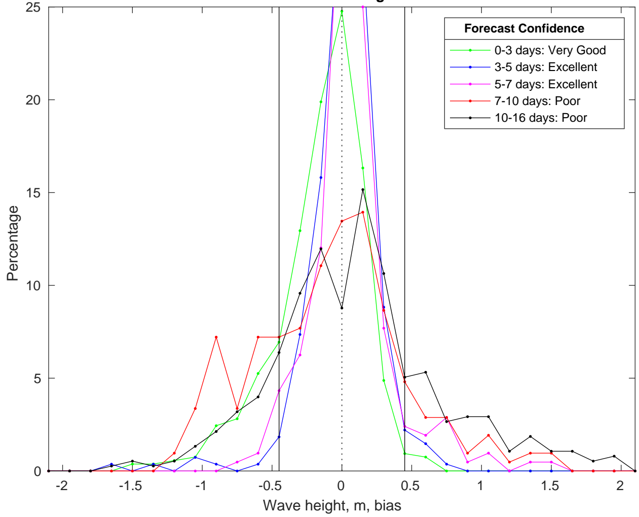
NDBC 41004 vs GFS Waves Bias Histogram: 08-Feb-2025
