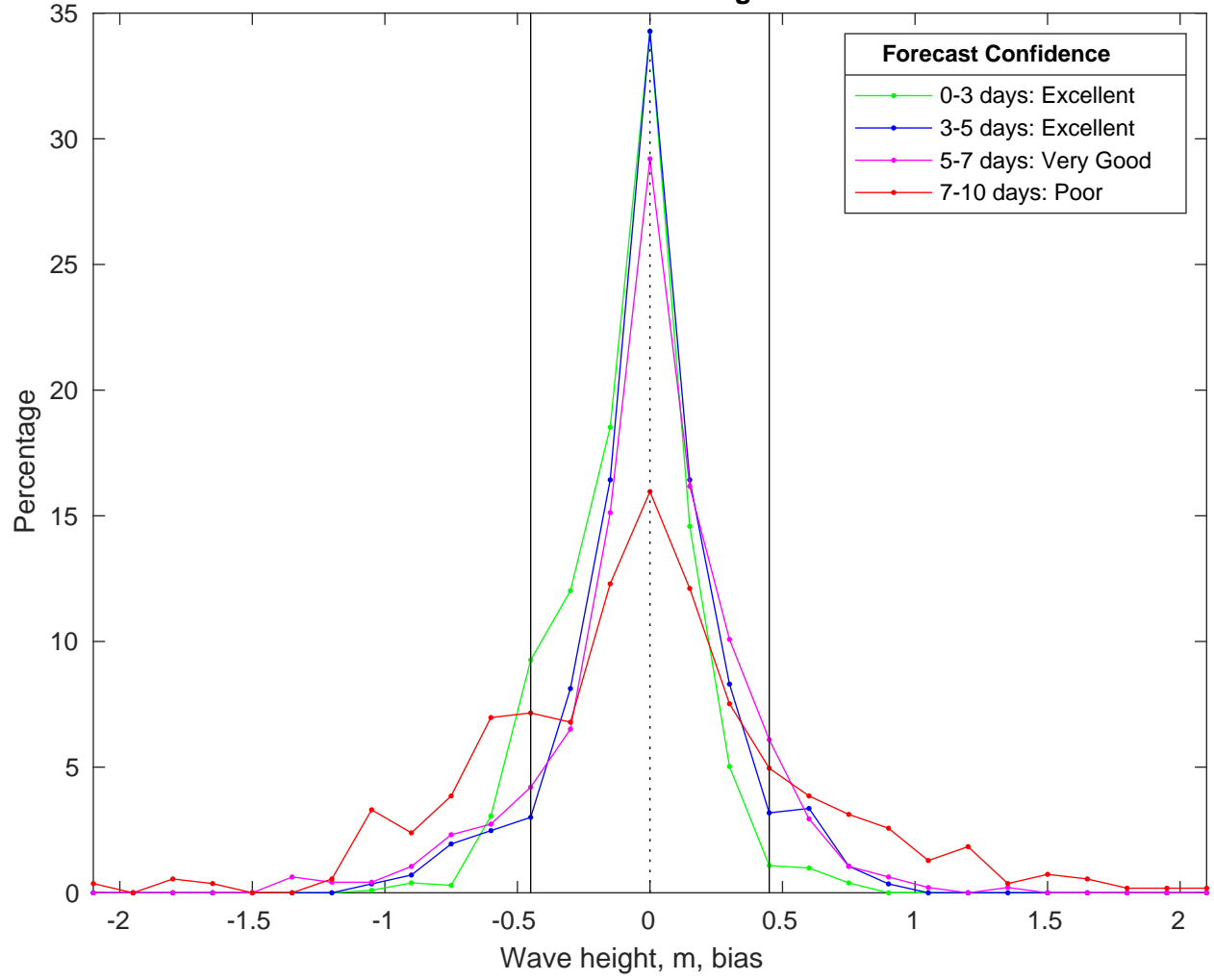
NDBC 41013 vs CMEMS Waves Bias Histogram: 08-Feb-2025
