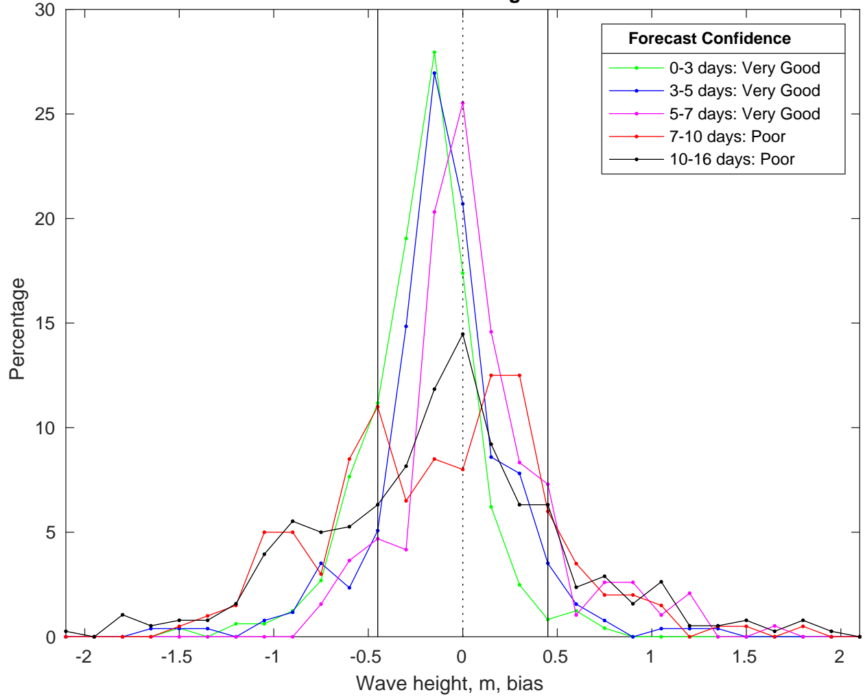
NDBC 41013 vs GFS Waves Bias Histogram: 08-Feb-2025
