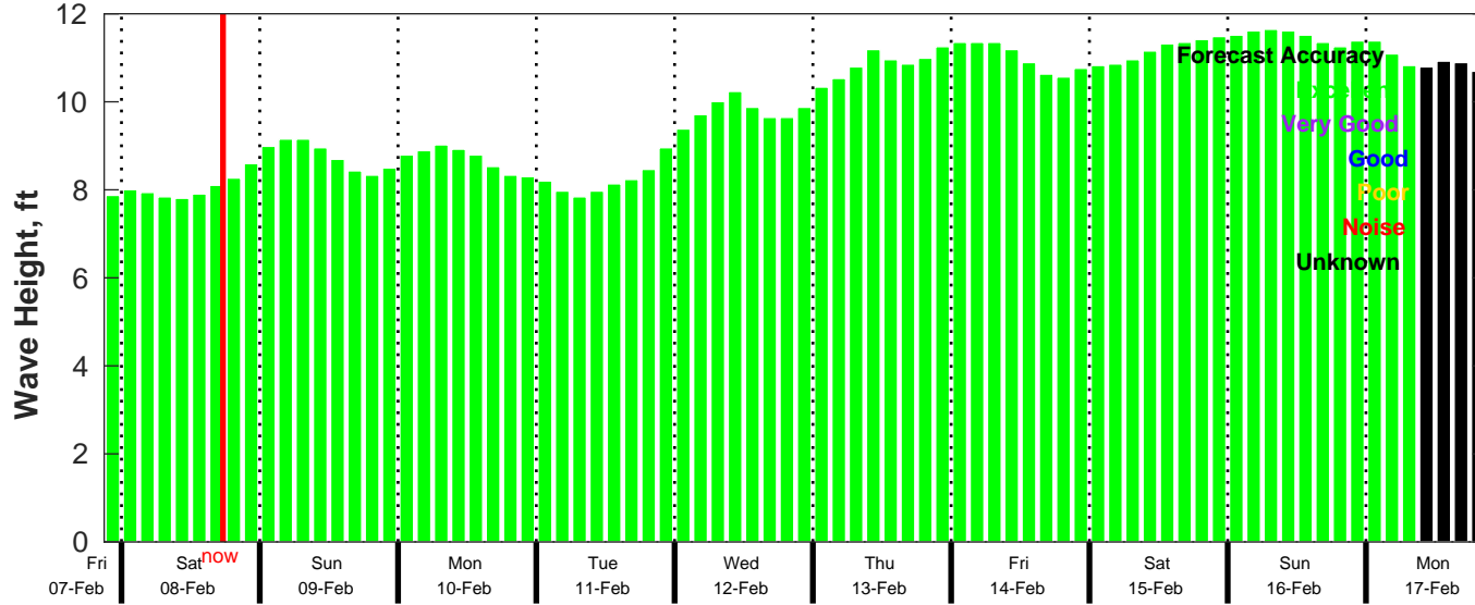
CMEMS Wave Forecast for NDBC 41040 from 07-Feb-2025 21:00:00 to 17-Feb-2025 21:00:00
