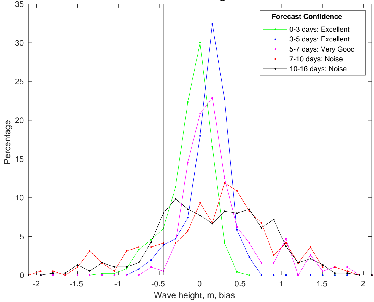
NDBC 42019 vs GFS Waves Bias Histogram: 08-Feb-2025
