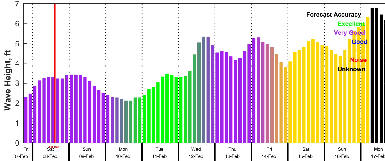
CMEMS Wave Forecast for NDBC 42019 from 07-Feb-2025 18:00:00 to 17-Feb-2025 18:00:00
