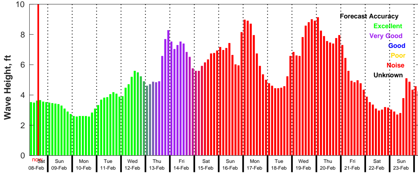
GFS Wave Forecast for NDBC 42019 from 08-Feb-2025 06:00:00 to 24-Feb-2025 06:00:00
