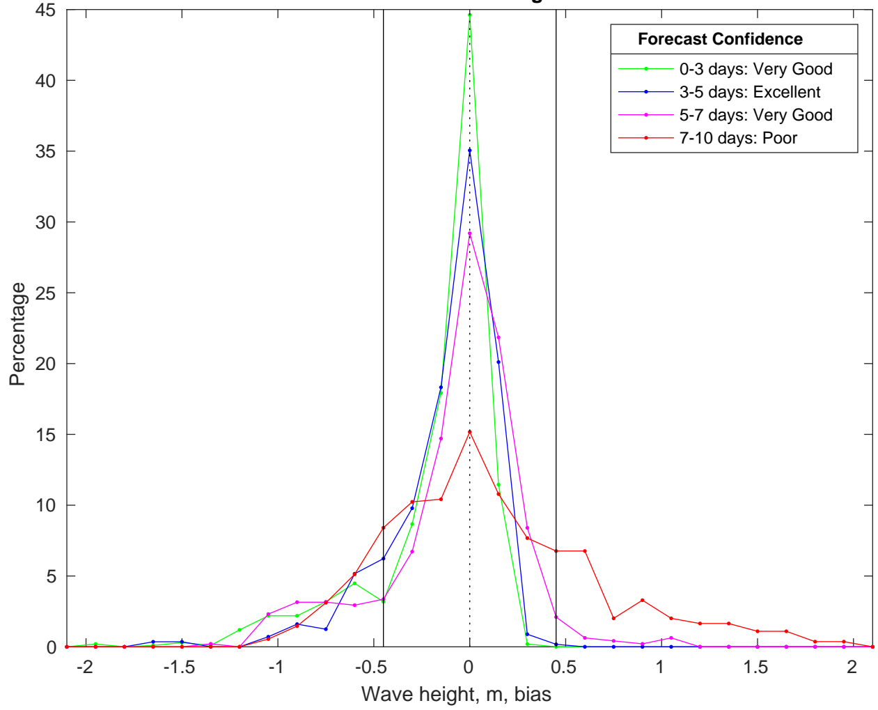
NDBC 42020 vs CMEMS Waves Bias Histogram: 08-Feb-2025
