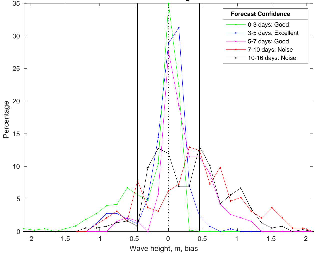
NDBC 42020 vs GFS Waves Bias Histogram: 08-Feb-2025
