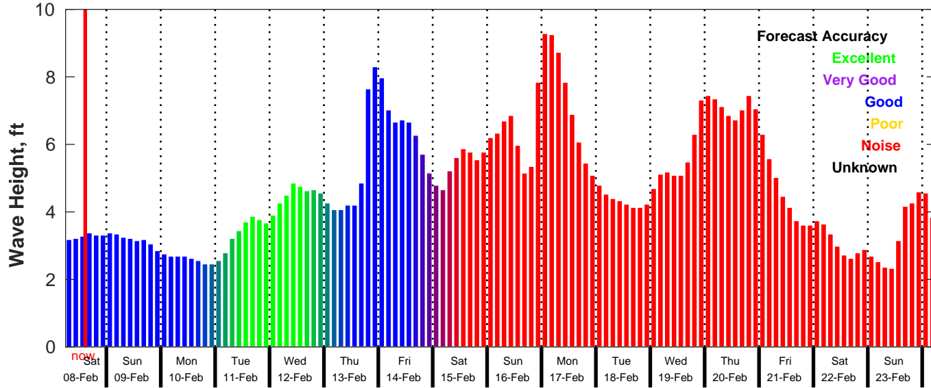
GFS Wave Forecast for NDBC 42020 from 08-Feb-2025 06:00:00 to 24-Feb-2025 06:00:00
