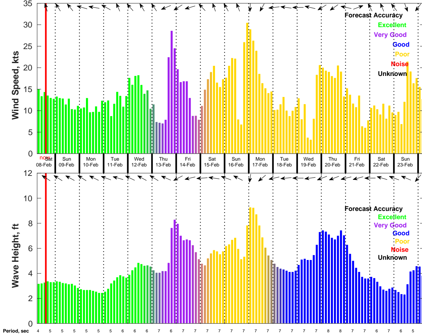
Wind & Wave Forecast for NDBC 42020 from 08-Feb-2025 06:00:00 to 24-Feb-2025 06:00:00
